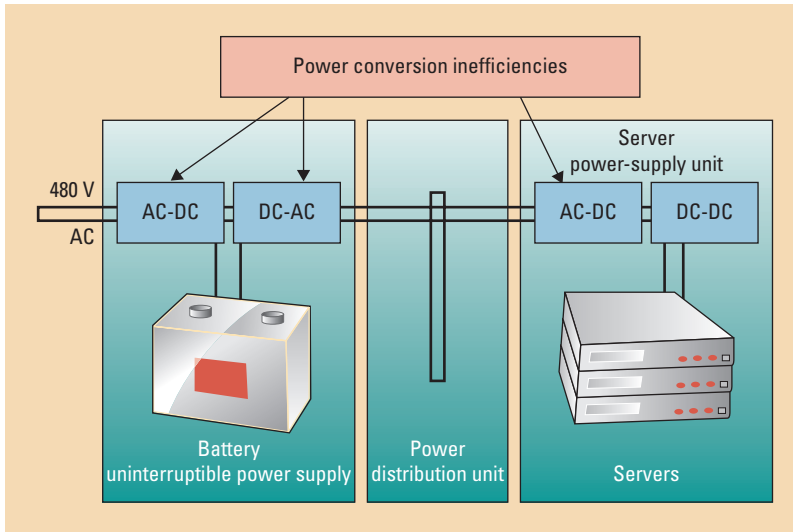
Figure 3. Traditional datacenter power architectures convert power between AC and DC at least three times. Converting datacenters to run on DC power only can reduce server power supply consumption and cooling requirements.
